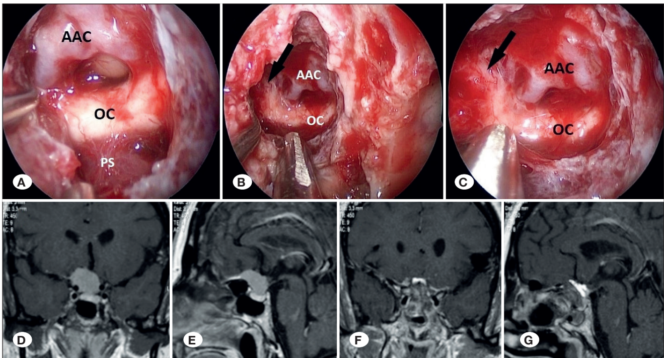
Figure 6: A) Evacuation of the optic canal invasion part of the tumor B) Evacuation of the optic canal inferomedial invasion. Black arrow indicates right optic nerve C) After evacuation of the optic canal invasion part of the tumor. Right optic nerve appears crushed (black arrow) D) Preoperative coronal T1-contrast-enhanced MR image of same patient E) Preoperative sagittal T1-contrast-enhanced MR image of same patient F) Postoperative coronal T1-contrast-enhanced MR image of same patient G) Postoperative sagittal T1-contrast-enhanced MR image of same patient. OC: Optic chiasm, AAC: Anterior artery complex, PS: Pituitary stalk.
