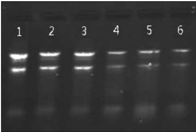
Figure 1: RNA Integrity and DNA contamination test by Denaturing Agarose Gel Electrophoresis.
