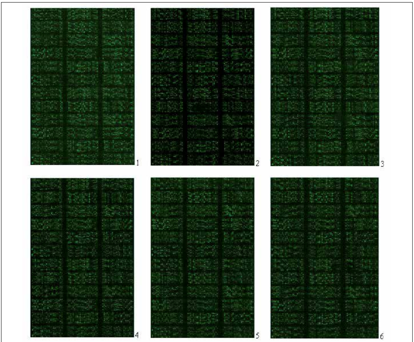
Figure 2: miRNA chip figures. Samples 1-3 were tumor tissue and Samples 4-6 were the corresponding negative controls.
