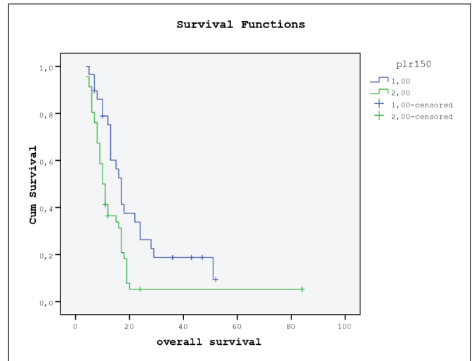
Figure 2: OS for PLR>150 and PLR \leq 150 patients.
