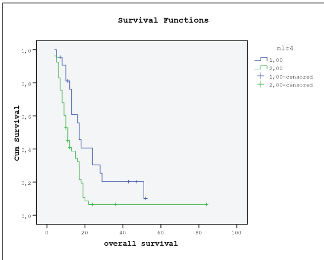
Figure 3: OS for NLR>4 and NLR≤4 patients.
