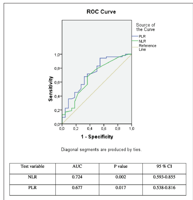
Figure 1: ROC curves for NLR and PLR.
